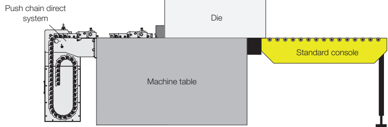
Combination of push chain direct system with standard carrying console
